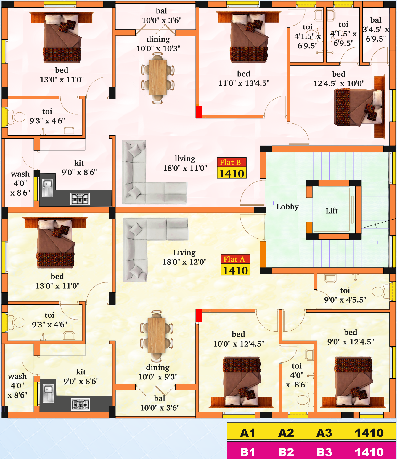
TYPICAL FLOOR PLAN [ I, II & III ]
